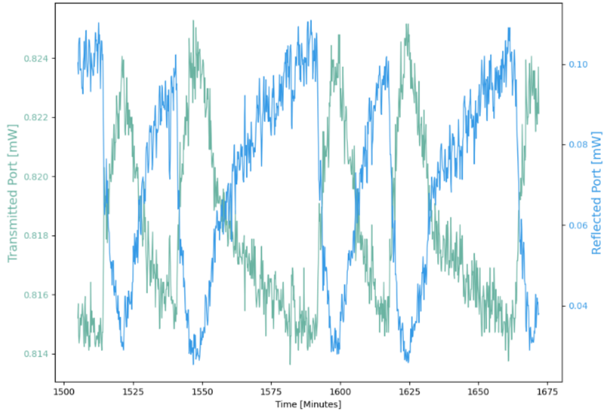
Laser Output PBS Ports, Oct 11th Over weekend
