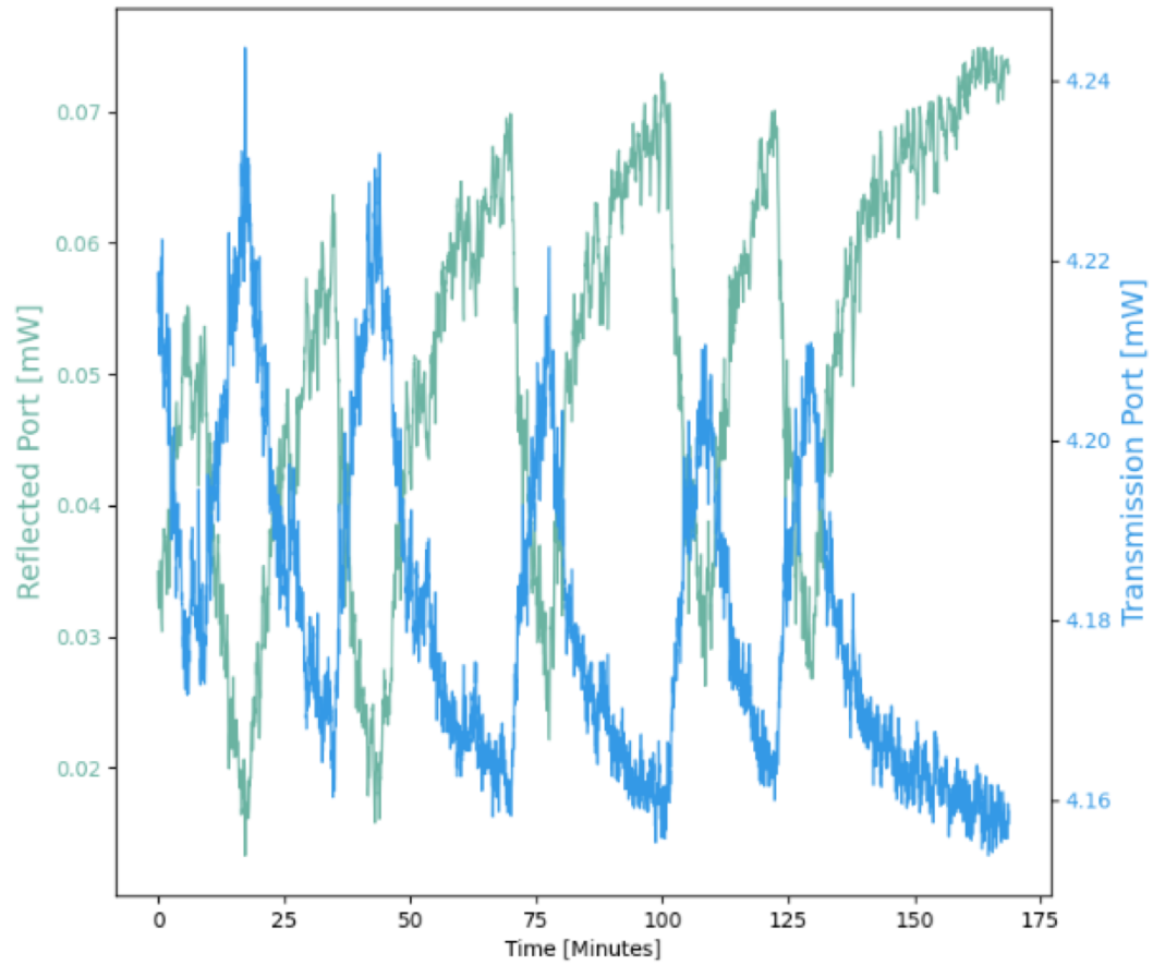
Laser Output PBS Ports, Oct 7th Overnight
