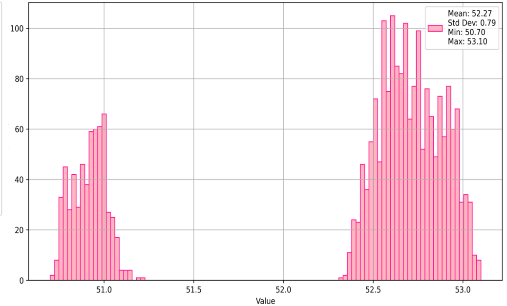
Histogram of Vbd_ROOM
