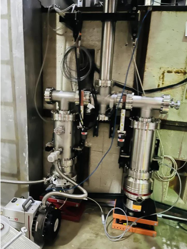
Insulation Vacuum Chamber (IVC) of the target magnet
