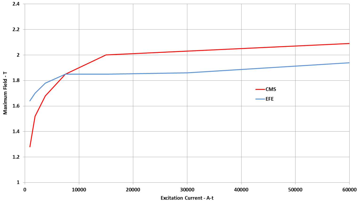
Maximum Field at Inner Radius of SuperBIND Iron for Various Excitation Currents
