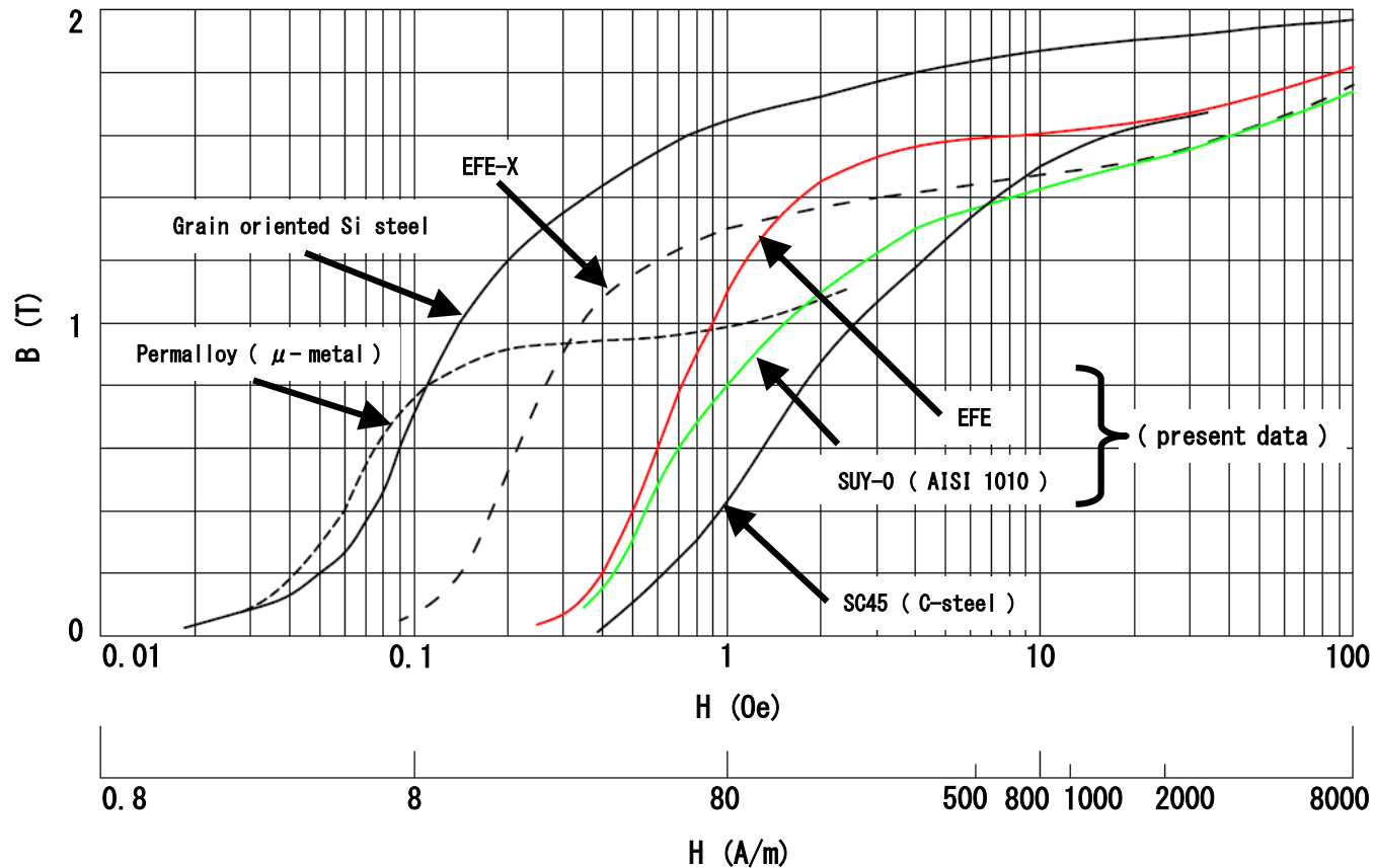
Fig. B-H curves of Ferro-magnetic materials for magnetic shielding at room temperature
