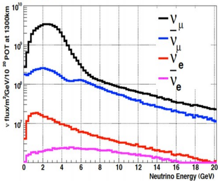
Neutrino Fluxes
