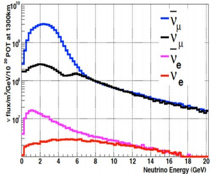
Anti-neutrino Fluxes
