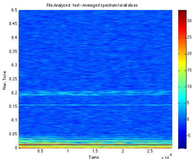
Figure 6: Closed-Loop (feedback on) spectrogram of figure 5 transient. The beam is TMCI unstable in these conditions, Q26 lattice, \nu_y = 0.185 \nu_s = 0.006 . The feedback control keeps the mode 1 and 2 unstable motion at the noise floor of the feedback receiver, or roughly 3 microns. A small amount of motion at mode zero is seen, this driven motion is reduced by the feedback gain.
