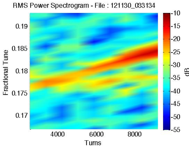
Figure 1: Open-loop vertical beam response chirp spectrogram measurement (no feedback). A 16 sample modulated excitation is driven by the kicker unto the SPS beam for 10,000 turns. The chirp excitation passes through the mode zero tune of 0.177 at turn 4000, and then the mode 1 upper synchrotron sideband at turn 8000 (Q20 lattice). The color code shows the amplitude of the motion for the detected signal.
