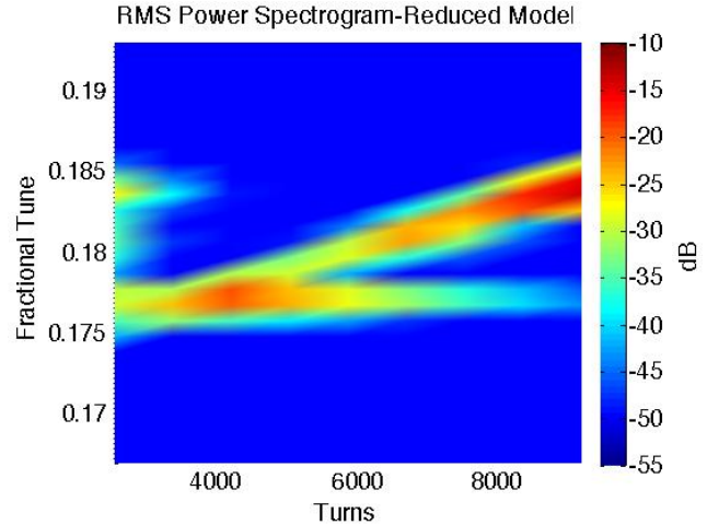
Figure 2: Beam motion spectrogram response for the reduced beam model (same excitation as figure 1). Comparing with the physical measurement we see very close agreement between the oscillation frequencies and the amplitudes of the excited motion.
