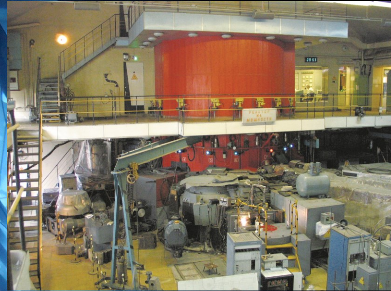
Source of thermal neutrons is a nuclear experimental reactor IR-8 in NRC KI with neutron flux of no less than 10^{12} \text{ cm}^{-2}\text{c}^{-1} ;
